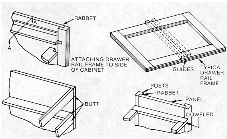
Figure 3-81. Drawer supports, or rail frames, are integral parts of case construction. Some typical assembly methods are shown here. Many rail frames are done with thin inset plywood panels so they serve as dust guards between drawer sections.
